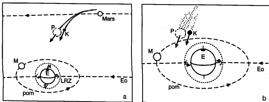
Fig 5.3ab. Phaeton's path close to the Earth.
